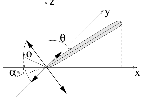
Fig. 1. Schematic diagram showing a bipolar outflow system (two possible directions shown by the thick, double arrows) ejected from a source located at the tip of an elephant trunk (grey, elongated structure at an angle \theta with respect to the z -axis). The z -axis lies along the line of sight, the xy -plane is parallel to the plane of the sky, and the x -axis is located along the plane of the sky projection of the elephant trunk. The outflow axis is perpendicular to the axis of the elephant trunk, and can be rotated at an angle \phi around the elephant trunk axis (with the outflow axis on the xz -plane for \phi = 0 ). The angle \alpha is measured between the x -axis and the projection of the outflow axis on the xy -plane.
