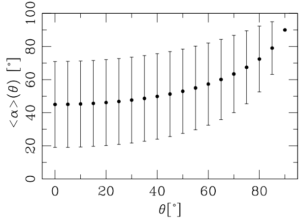
Fig. 3. The mean value (dots) \langle \alpha \rangle (\theta) and standard deviation (error bars) \sigma(\theta) (see equations 5 and 6, respectively) derived for the D_\theta(\alpha) distributions (see equation 3) as a function of the angle \theta between the elephant trunks and the line of sight. For \theta = 90^\circ , we have \langle \alpha \rangle = 90^\circ and \sigma = 0 .
