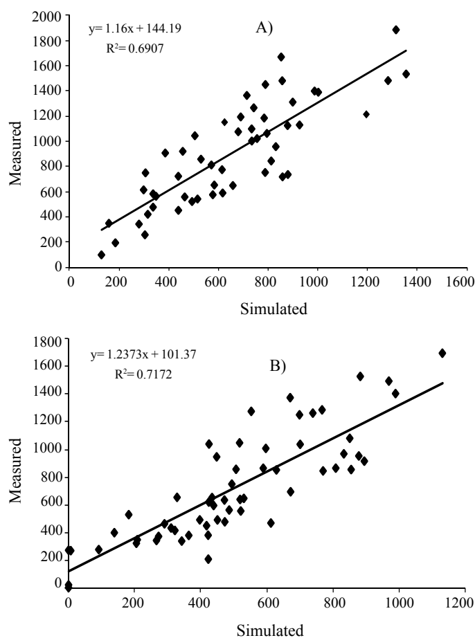
Figure 3. Comparison of simulated and observed bean yield under dryland conditions during 2006 (A) and 2007 (B) spring-summer growing seasons in the state of Zacatecas, Mexico.
