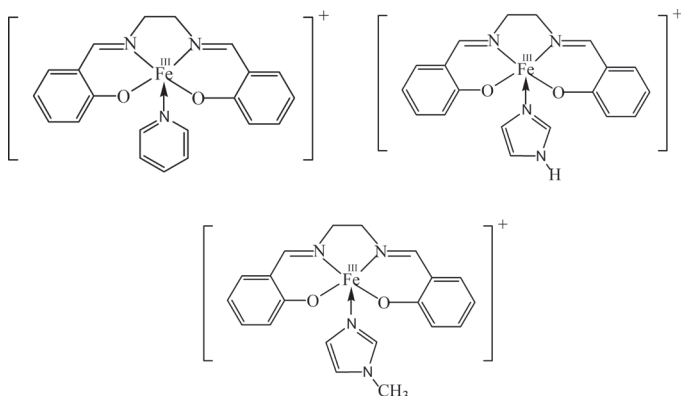
Structure 2. Adduct formed between [\text{Fe}^{\text{III}}(\text{salen})]^+ and pyridine bases.
