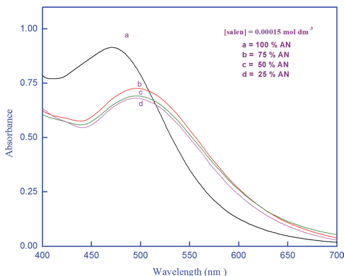
Fig. 2. Overlay spectrum of iron(III)-salen complex in different solvent mixtures.
