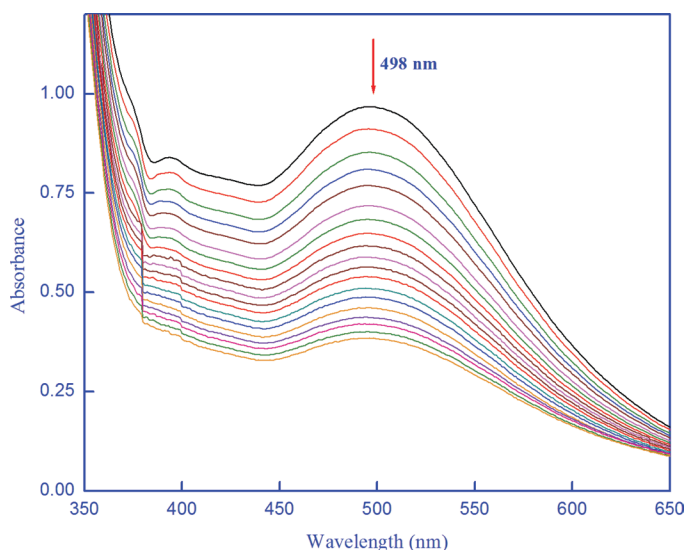
Fig. 1. Absorption spectral changes in the reaction of iron(III)-salen complex ( 2 \times 10^{-4} \text{ mol dm}^{-3} ) with TDGA ( 5 \times 10^{-2} \text{ mol dm}^{-3} ) in 50% aqueous acetonitrile medium at 30 °C. The spectra were recorded for 900 sec (every 45 sec) after mixing.
