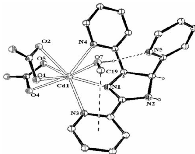
Fig. 3. Perspective view of the molecular structure of the monomeric complex [Cd(L)(NO 3 ) 2 (MeOH)] ( 1 ), showing the numbering scheme and the thermal ellipsoids at the 50% probability level (dashed lines indicate the H-bonding and a weak CH...π interaction).
