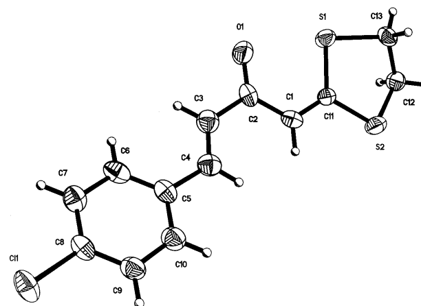
Figure 1. ORTEP drawing of ligand 3 . Thermal ellipsoids at 30% probability level.
