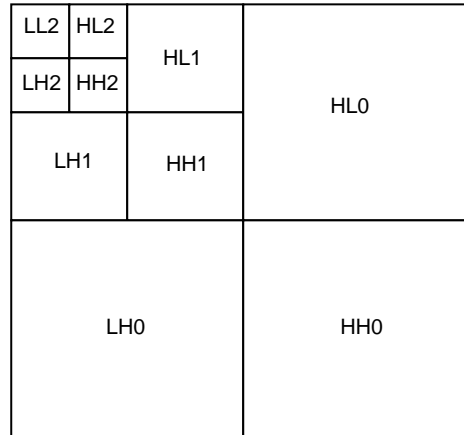
Figure 2. Three levels of wavelet decomposition
