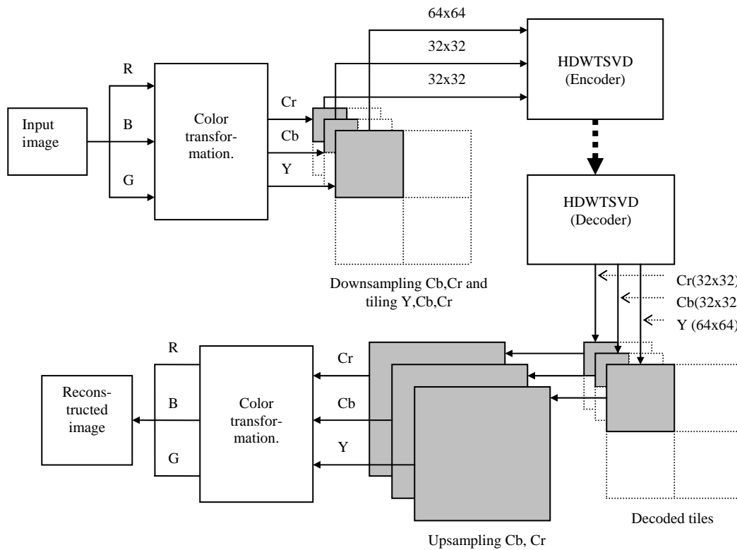
Figure 7. The HDWTSVD system for color images
