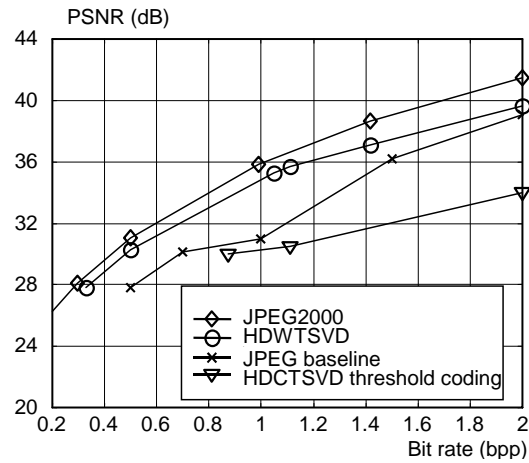
Figure 9. Comparison of the HDWTSVD with JPEG2000, JPEG baseline, and HDCTSVD using threshold coding for the Barbara image
