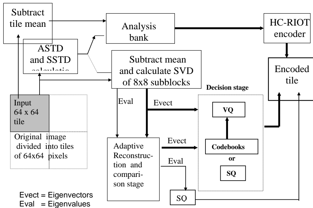
Figure 5. The HDWTSVD encoder
