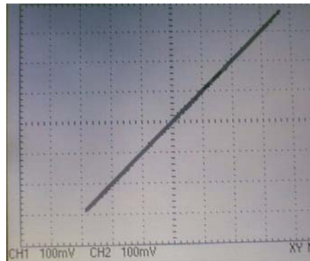
Figure 4. Synchronization between the master and slave circuits: x_1(t) of the master (horizontal axis) versus \xi_1(t) of the slave (vertical axis)
