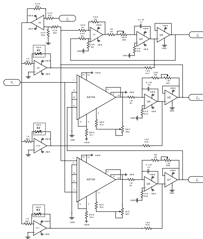
Figure 3. Experimental set-up of Generalized Hamiltonian systems and observer approach to synchronize the Lorenz circuit
