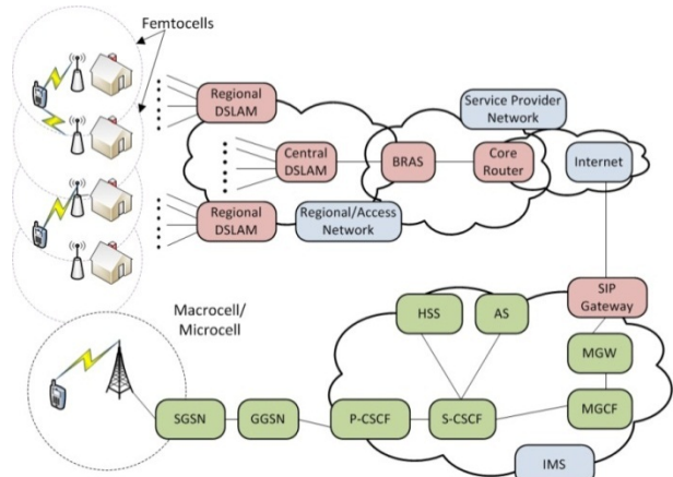
Figure 1. A general femtocell deployment architecture.
