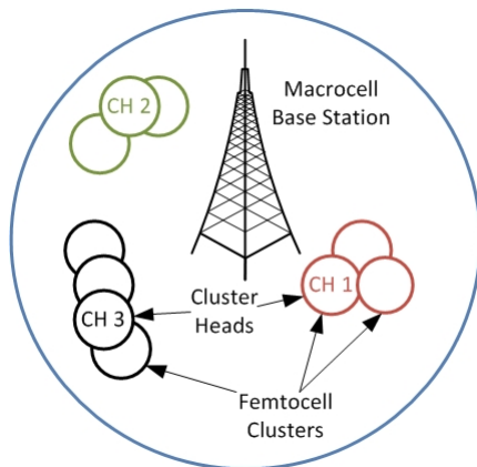
Figure 9. Clustered femtocell network.
