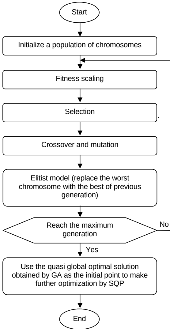
Figure 1. Flowchart of the hybrid GA-SQP.
