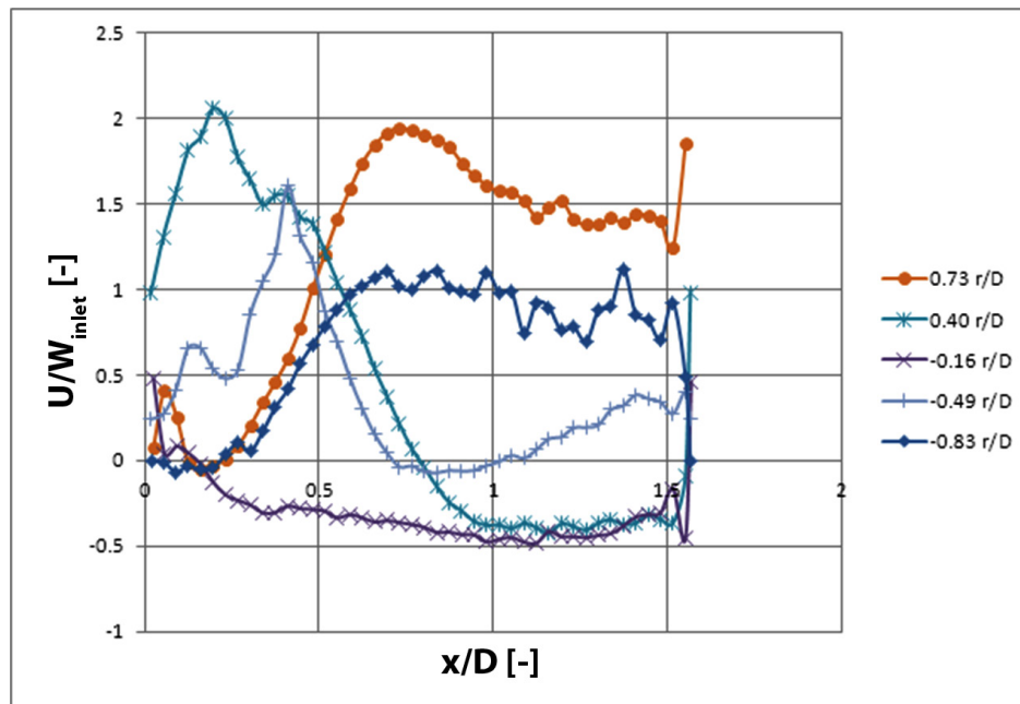
Figure 12. Axial velocities at different radial positions, plane 0-180°.
