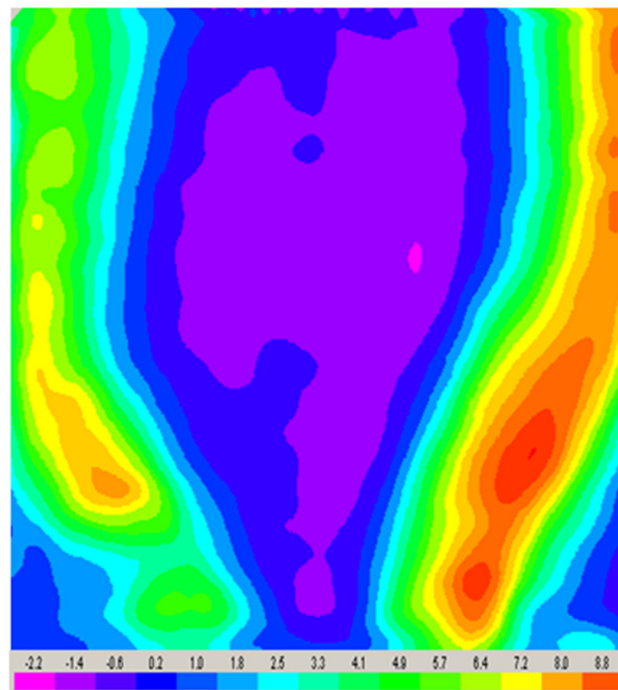
Figure 7. Axial velocity, U, plane 0-180°.
