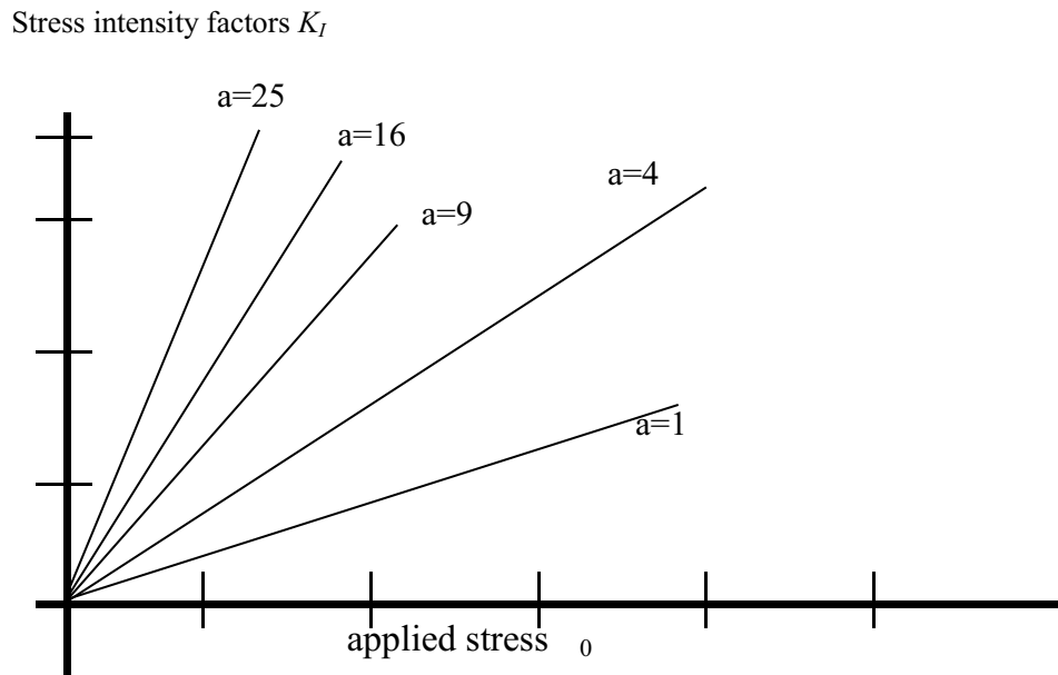
Figure 3. K_I stress intensity factor as function of applied stress applied with breakage length a as a parameter [2]
