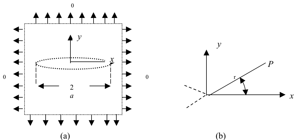
Figure 2. 2a long crack on an infinite plate subject to biaxial load
