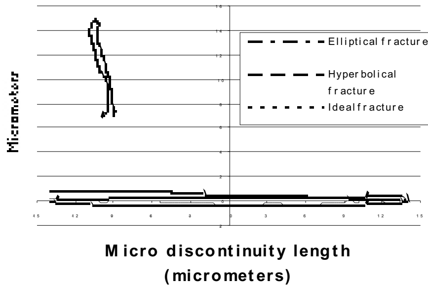
Figure 5. Graphic representation of micro discontinuities shown in figure 4
