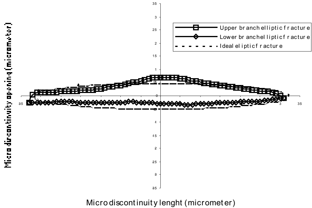
Figure 9. Graphic representation of the micro discontinuity in figure 8
