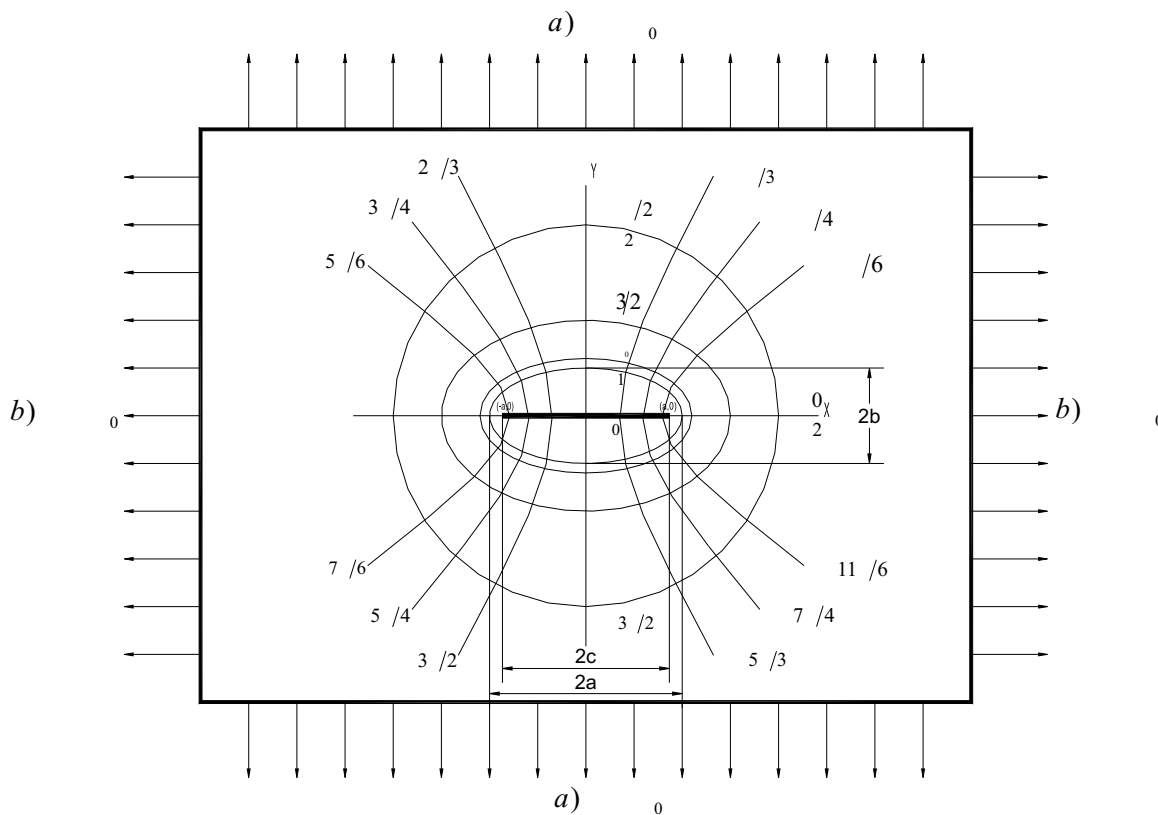
Figure 1. Elliptical micro-discontinuity on a plate with a) perpendicular \sigma_0 uniaxial load at x, and b) parallel \sigma_0 uniaxial load at x
