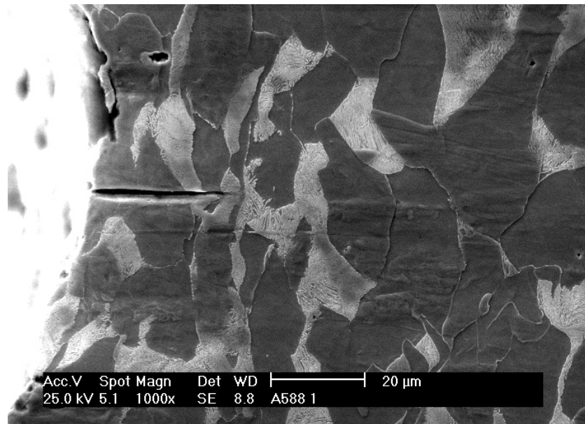
Figure 4. Elliptical micro discontinuity and generation of the micro discontinuity perpendicular to such, with probable hyperbolic behavior
