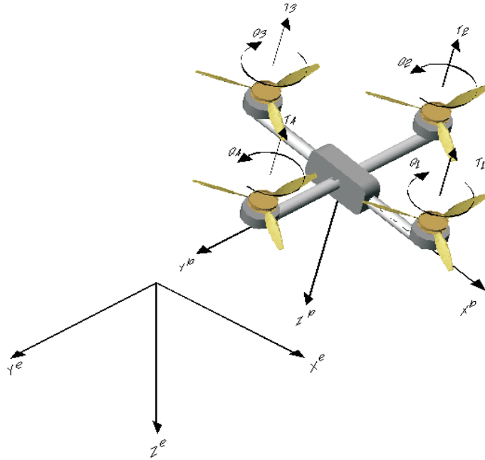
Figure 1. Rotary wing vehicle
