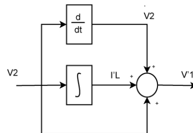
Figure 3. Block diagram of the circuit to estimate the states V_1 and I_r .
