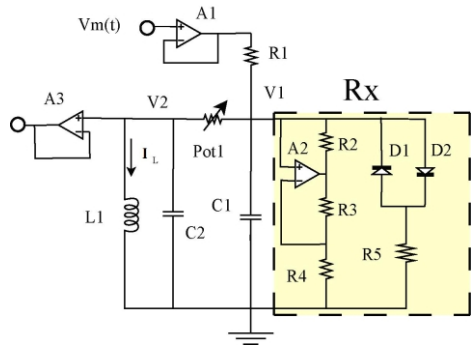
Figure 2. The electronic circuit of the transmitter block. The component values employed are R_1 10k , R_2 R_3 220 , R_4 750 , R_5 1.2 , Pot1 5k , C_1 10nF, C_2 100nF, L_1 18mH. The diodes D_1 and D_2 are 1N914, and the operational amplifiers are TL-082.
