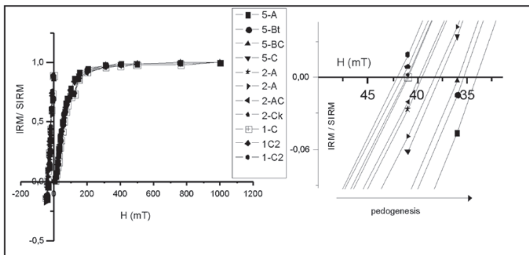
Figure 4. IRM acquisition curves for selected samples from different horizons of the studied profiles. The detail at right shows the variation of Bcr related to pedogenesis degree.
