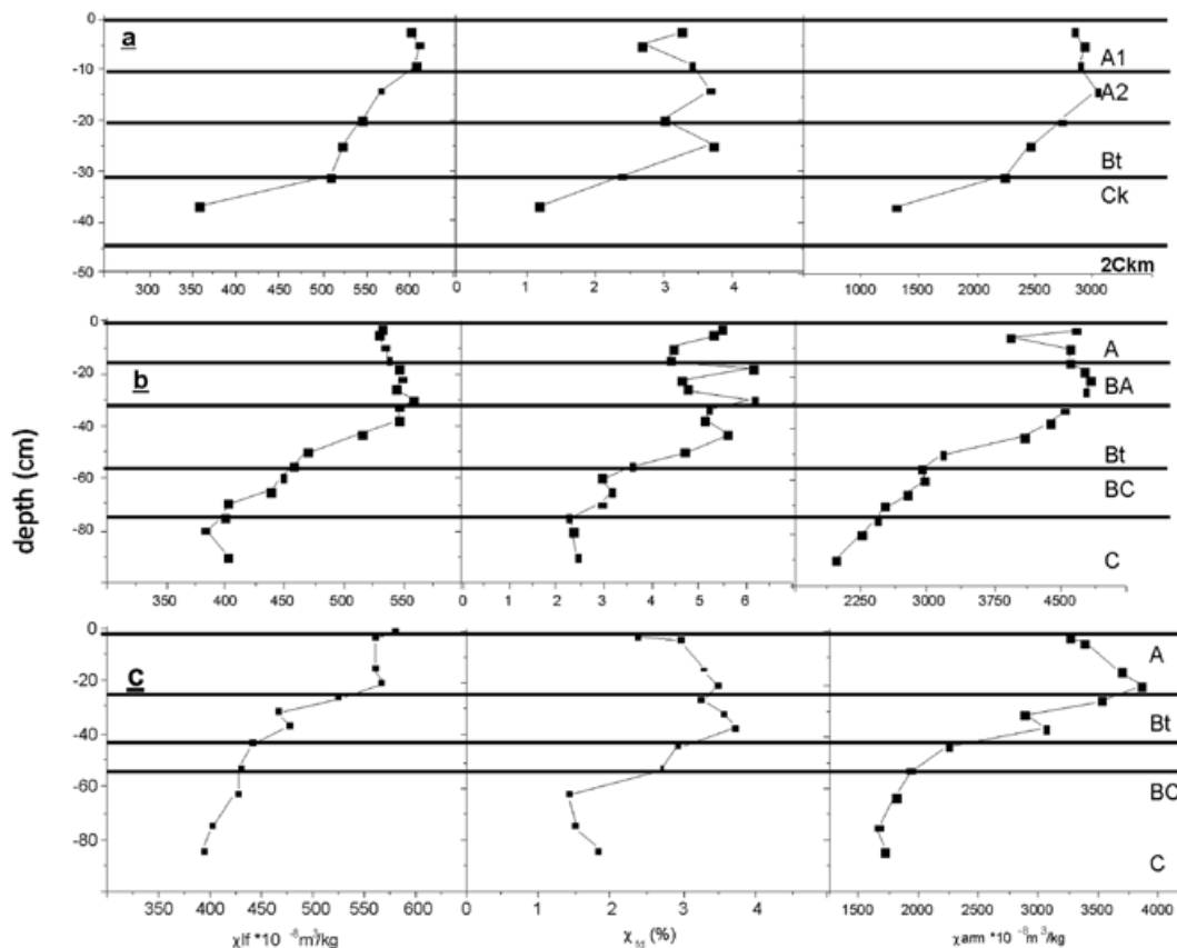
Figure 3. Magnetic properties for the soils of subhumid climate: Lithic Argiustoll P3 (a) and Typic Argiudolls P4, P5 (b, c). Soil horizons are indicated at right.
