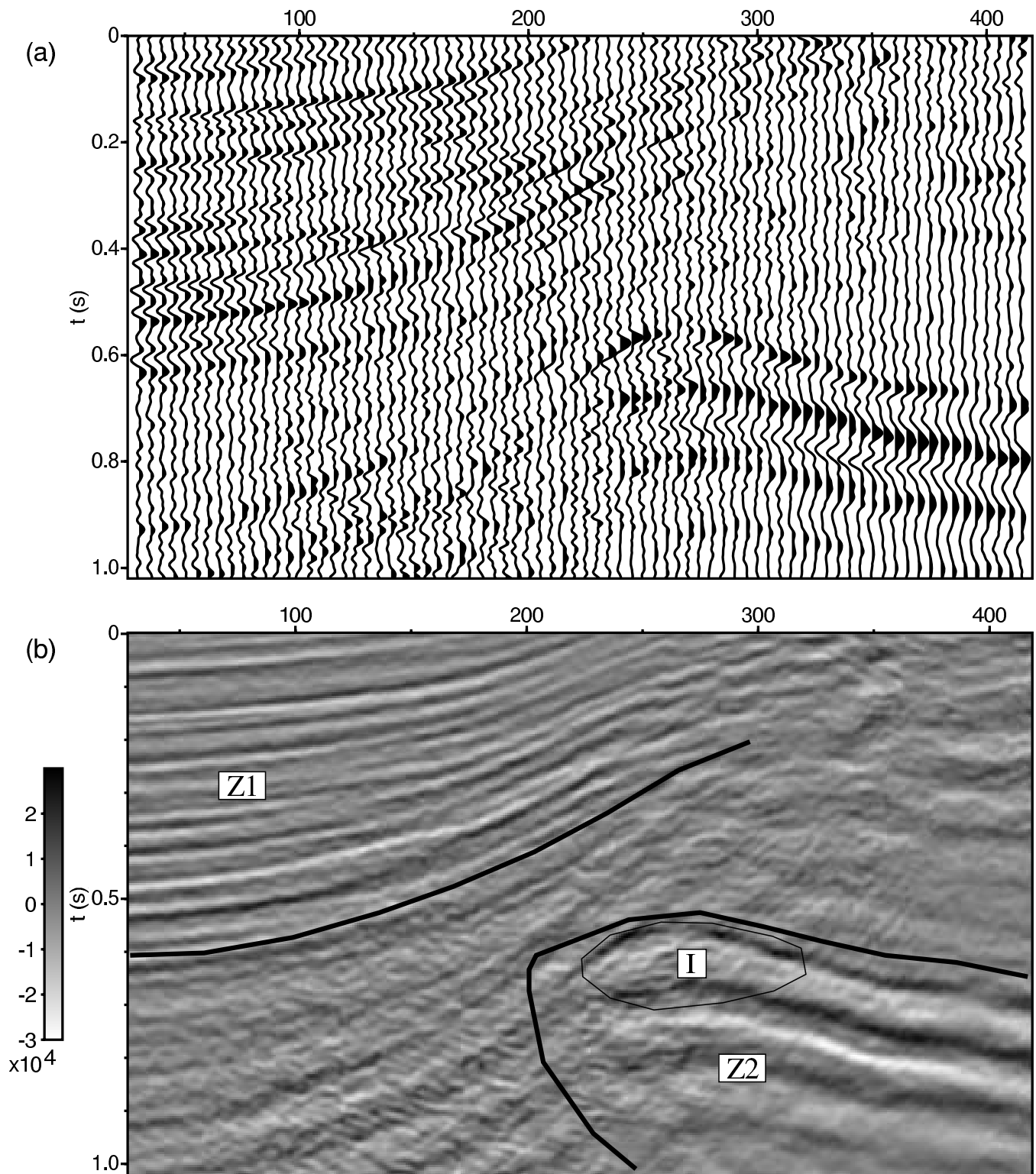
Fig. 1. A seismic section: (a) wiggle-trace plot, (b) image plot.
