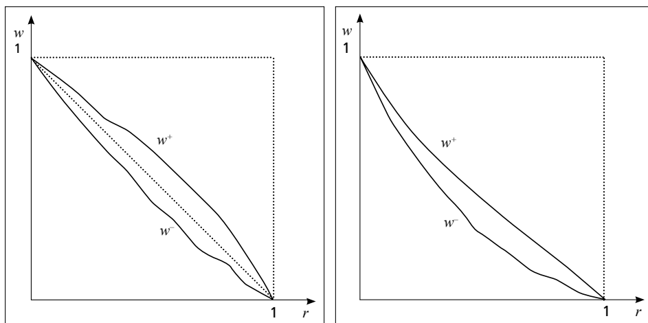
Figure 2. Upper and lower bounds for wages when R = 1 , m = 1 , t = 0 and 1 = 1_R Figure 3. Upper and lower bounds for wages when R = 1 , m = 1 , t = 1 and 1 = 1_R
