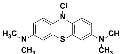
Methylene blue Substance D
