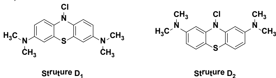
Figure 5. Possible structures of substance D.
