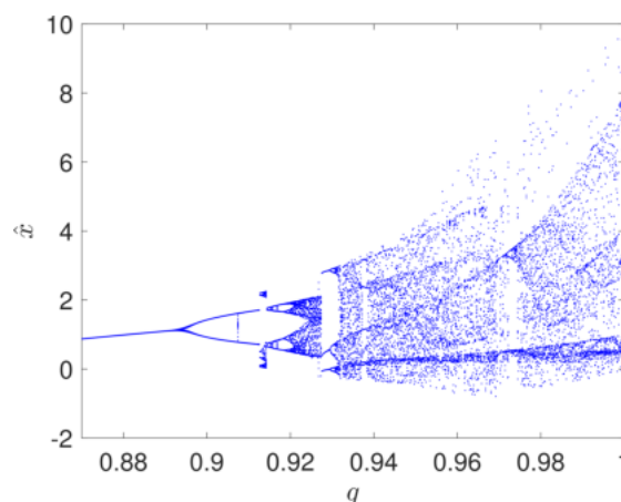
Fig. 1. Bifurcation diagram for the fractional order q
