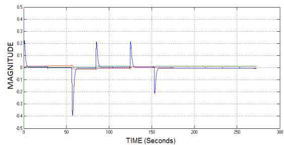
Fig. 6. Position error between system and reference, red: X position (cm), green: Y position (cm), blue: angle (radians) (Test 1)
