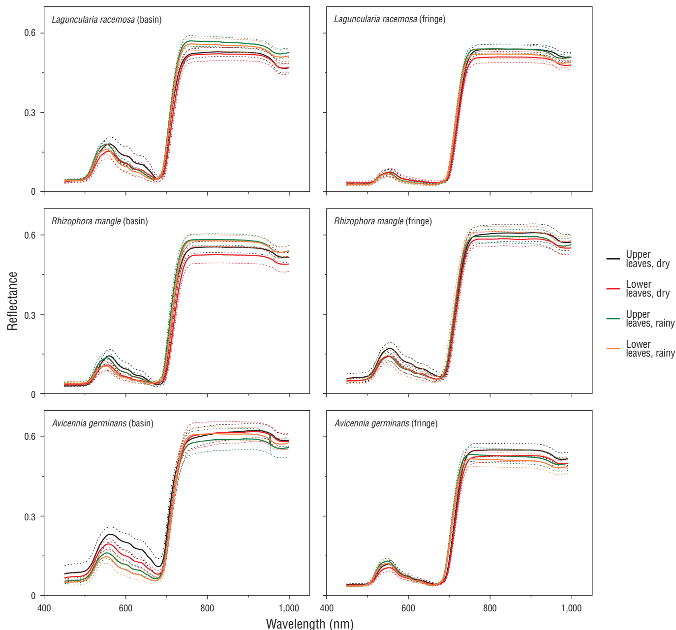
Figure 2. Average reflectance ( n = 30 , solid line) and first standard deviation (dashed line) for leaves of 3 mangrove species in basin and fringe forests.
