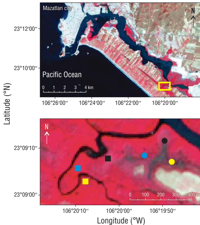
Figure 1. Location of the mangrove forest study area (yellow rectangle) on the southwestern section of the Urias coastal lagoon, Pacific coast of Mexico (enhanced near-infrared, red, and green bands from Sentinel-2; 26 January 2017). Filled circles indicate the sampling locations in the basin and filled squares the sampling locations in the fringe zone. Colors indicate mangrove species: Avicennia germinans (black), Laguncularia racemosa (yellow), and Rhizophora mangle (blue).
