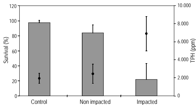
Figure 3. Survival rates of the polychaete Scolecopsis texana (bars) and total petroleum hydrocarbon (TPH) concentrations in the sediments (dots) during each of the toxicity assay treatments with sediments impacted and not impacted by the refinery.
