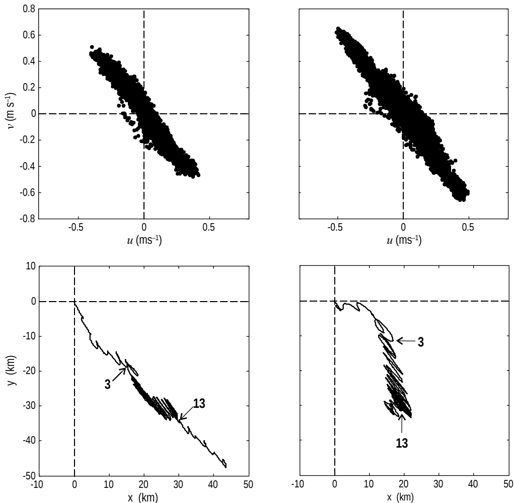
Figure 2. Velocity components ( u , v ) measured at site W3 at 5 and 15 m above the seabed during a fortnightly cycle (upper diagrams), and progressive vectors at the same levels (lower diagrams). Neap tides occur at the beginning and end of the plots. The numbers indicate the days as of 11 August 1997.
