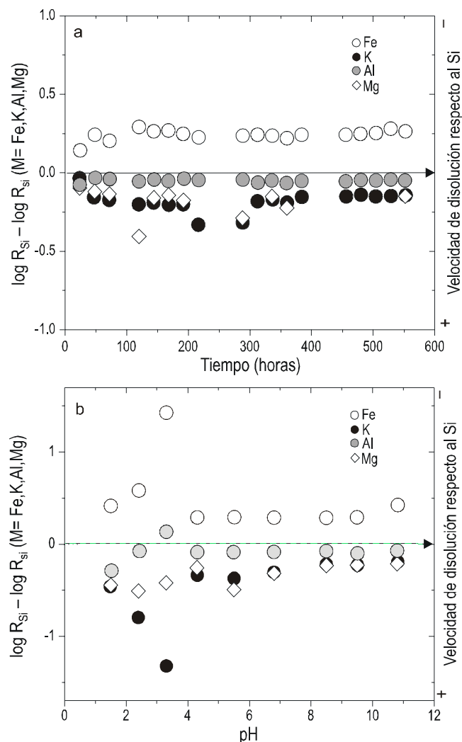
Figura 3. Determinación del rango de disolución congruente. \log R_{Si} - R_M = 0 indica disolución congruente. (a) En función del tiempo, a pH = 8.5, las velocidades se aproximan a un valor constante respecto al Si, siendo K > Mg > Al > Fe . (b) En función del pH se observa un intervalo de disolución incongruente a valores de pH < 4, asociado a la rápida liberación del K^+ . Figure 3. Determination of the range of congruent dissolution. \log R_{Si} - R_M = 0 indicates congruent dissolution. (a) As a function of time, at pH = 8.5, the rates are close to a constant value relative to Si, with K > Mg > Al > Fe . (b) As a function of pH, an incongruent dissolution range is observed at values of pH < 4, associated with the rapid release of K^+ .
