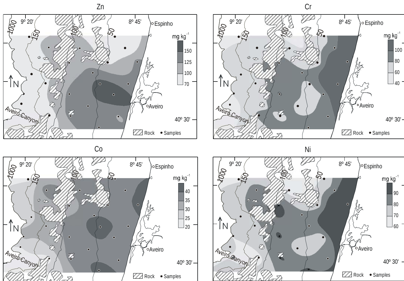
Figure 4. Distribution maps of the concentrations of Zn, Cr, Co and Ni, in the fine fraction of shelf sediments between Espinho and Aveiro (Portugal).
