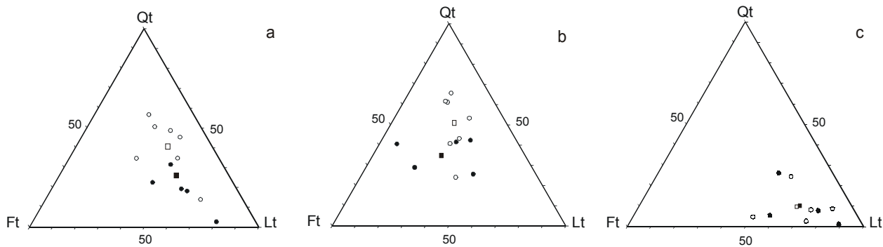
Figure 4. Qt-Ft-Lt ternary plots of (a) beach ( n = 12 ), (b) dune ( n = 12 ) and (c) river sands ( n = 9 ). Trans-Mexican Volcanic Belt (TMVB) sands, \circ ; and Veracruz Embayment (VE) sands, \bullet . Average values of TMVB sands, \square ; and VE sands, \blacksquare . Figura 4. Diagramas ternarios Ct-Ft-Lt de las arenas de (a) playa ( n = 12 ), (b) duna ( n = 12 ) y (c) río ( n = 9 ). Arenas del Cinturón Volcánico Trans-Mexicano (CVTM), \circ ; y de la Cuenca Veracruzana (VE), \bullet . Valores medios de las arenas del CVTM, \square ; y de la CV, \blacksquare .
