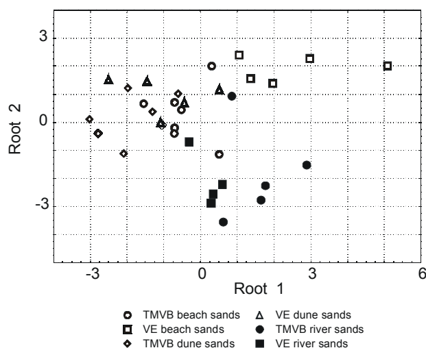
Figure 5. Canonical variate diagram for discriminant function scores ( n = 33 ): root 1 vs root 2.
