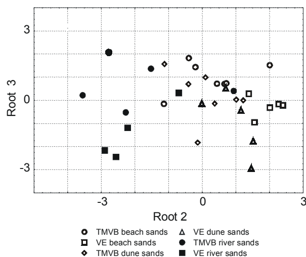
Figure 6. Canonical variate diagram for discriminant function scores ( n = 33 ): root 2 vs root 3.
