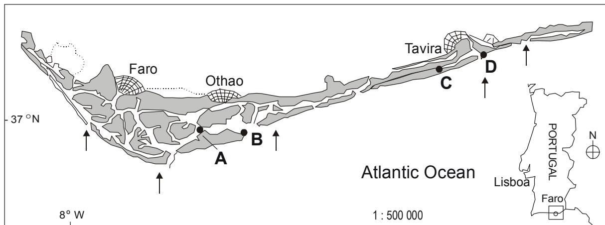
Figure 1. Ria Formosa and sampling stations A, B, C and D.
