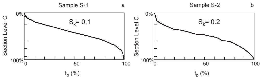
Figure 3. Abbot-Firestone curves and their corresponding skewness values calculated from roughness profiles recorded in the eroded zones of samples (a) S-1 and (b) S-2.
