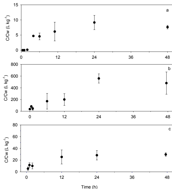
Figura 2. Curvas de cinética de C_{11} -SPC sobre sedimento (a) y las microalgas marinas Nannochloropsis gaditana (b) y Dunaliella salina (c). Figure 2. C_{11} -SPC kinetic curves on marine sediment (a) and microalgae, Nannochloropsis gaditana (b) and Dunaliella salina (c).
