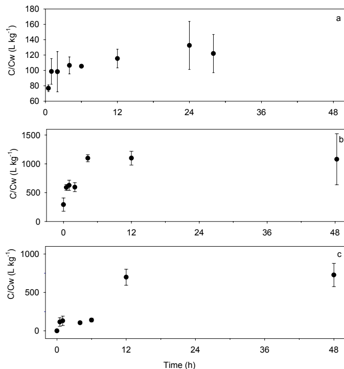
Figura 1. Curvas de cinética de C_{11} -LAS sobre sedimento (a) y las microalgas marinas Nannochloropsis gaditana (b) y Dunaliella salina (c). Figure 1. C_{11} -LAS kinetic curves on marine sediment (a) and microalgae, Nannochloropsis gaditana (b) and Dunaliella salina (c).
