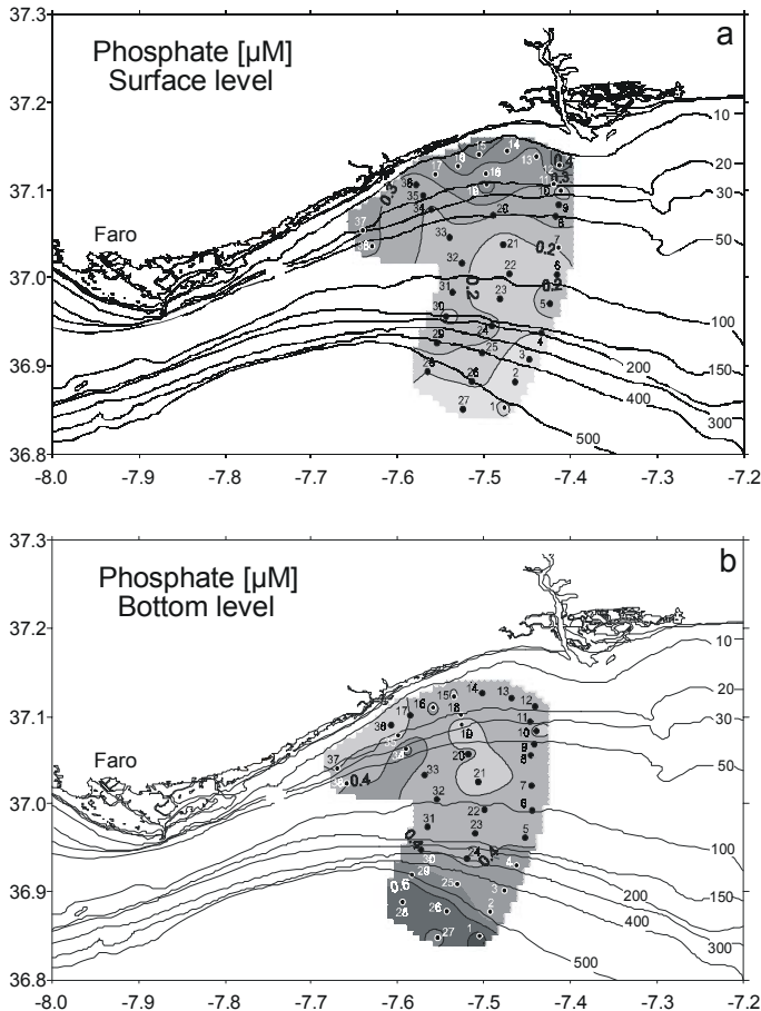
Figure 6. Distribution of phosphate concentrations ( \mu\text{M} ) at: (a) surface and (b) bottom.
