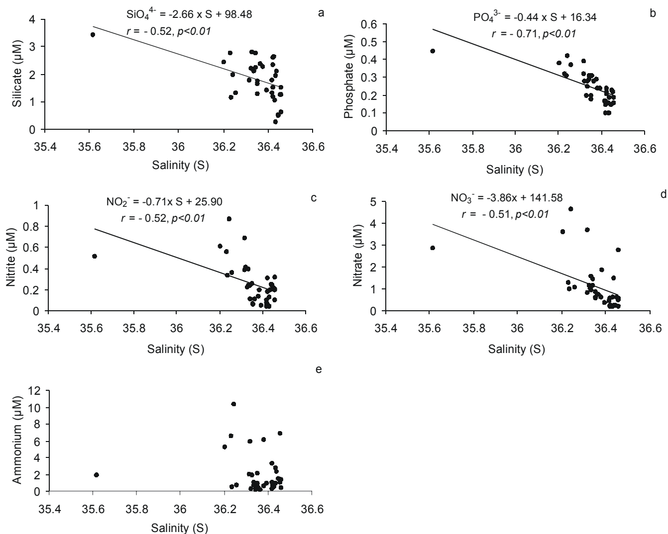
Figure 8. Relationship between concentration ( \mu\text{M} ) of: (a) silicate, (b) phosphate, (c) nitrite, (d) nitrate and (e) ammonium and salinity.
