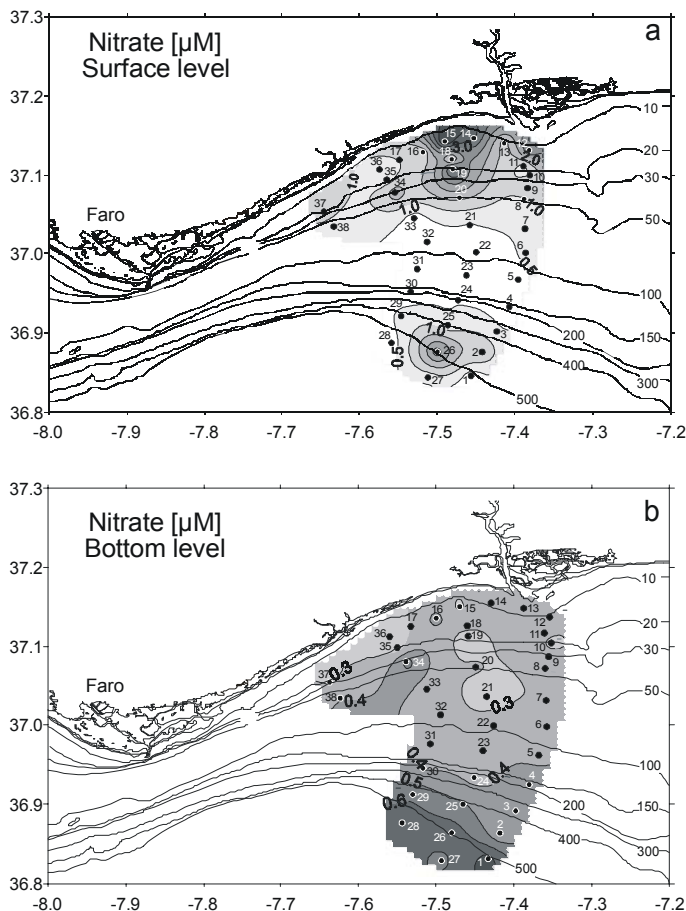
Figure 5. Distribution of nitrate concentrations ( \mu\text{M} ) at: (a) surface and (b) bottom.
