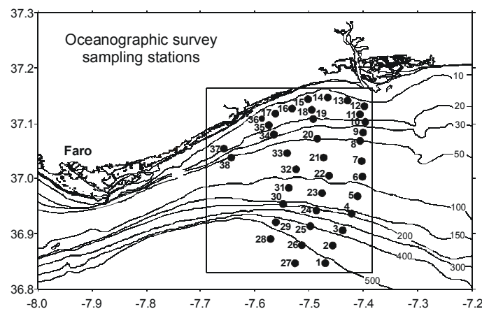
Figure 2. Location of the sampling stations.
