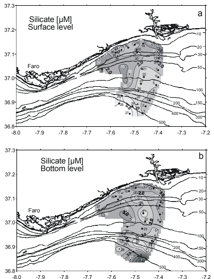
Figure 7. Distribution of silicate concentrations ( \mu\text{M} ) at: (a) surface and (b) bottom.
