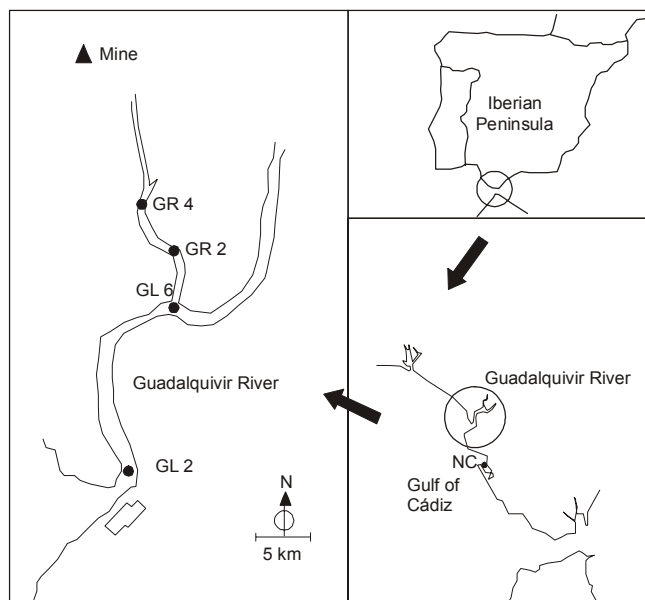
Figure 1. Map of the Guadalquivir estuary located in the Gulf of Cádiz, showing the general areas sampled and location of the sampling stations. The negative control (NC) used in the toxicity tests and for the toxic mud dilution (TM) is represented by the symbol ♦.
