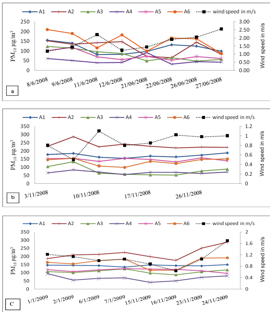
Fig. 3. a, b, c. Sample-to-sample and site-to-site comparison of the PM 10 mass concentration (left Y-axes) with associated wind speed (right Y-axes) at six sites in Talcher.
