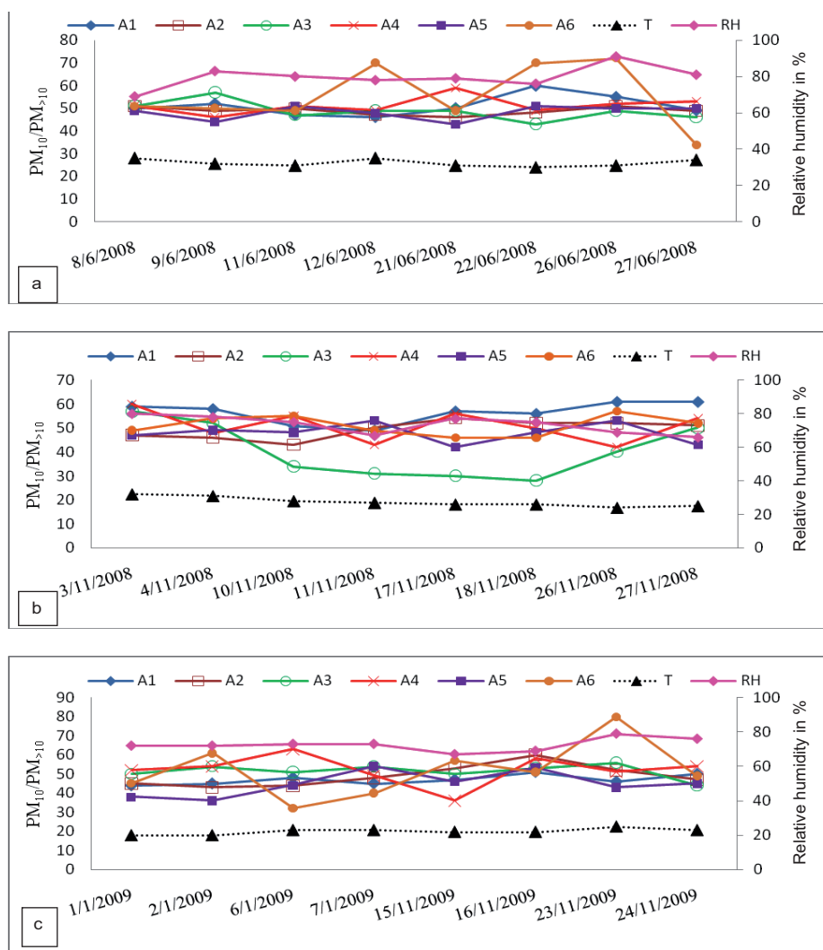
Fig. 4. a, b, c. Comparison of calculated PM_{10} to PM_{>10} ratio at six sites (left Y-axes) during this study.
