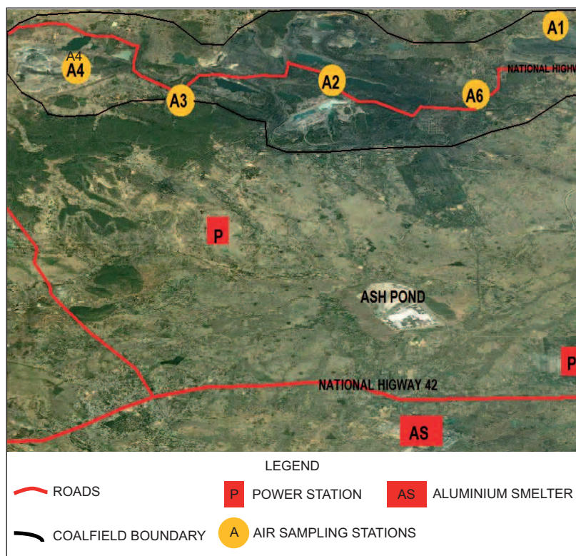
Fig. 2. Sampling stations and major industrial locations of the study area.
