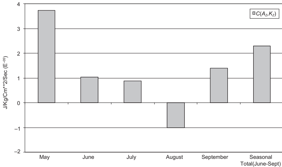
Fig. 3. Monthly and seasonal total C(A_Z, K_Z) : decadal average (2000-2009).
