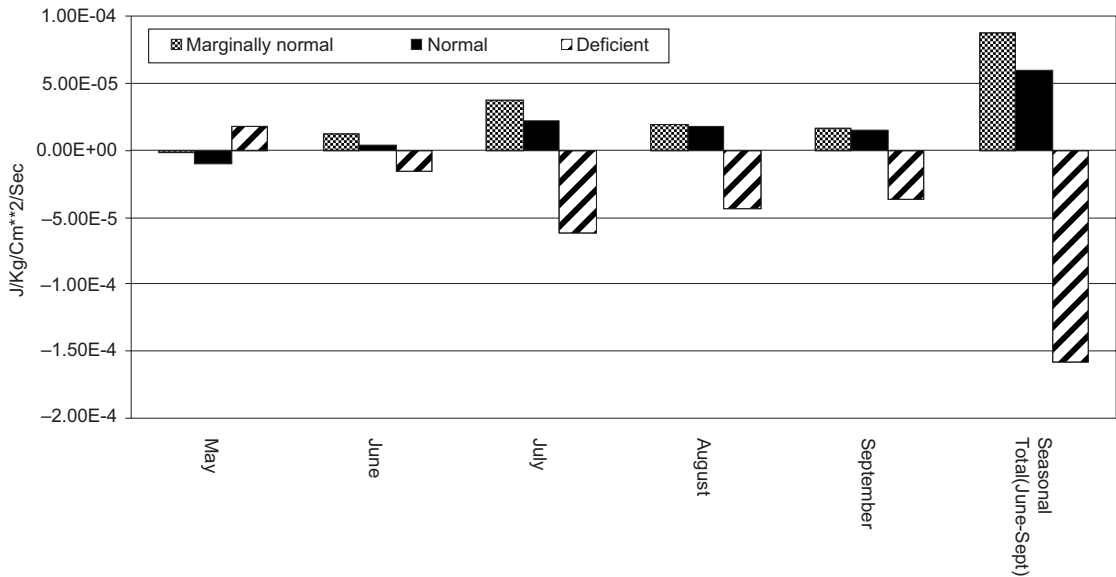
Fig. 7. Composite anomaly of monthly/Seasonal total C(A_z, K_z) .
