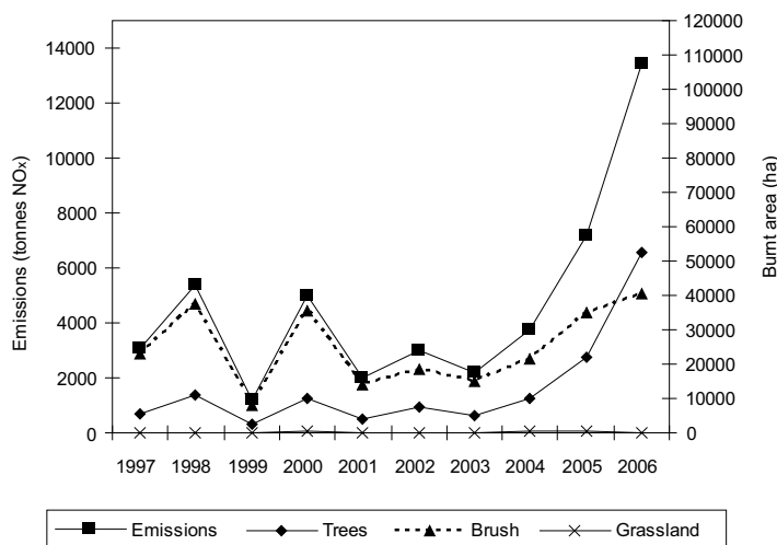
Fig. 1. NO x emissions associated with fires (left axis) and areas of trees, brush and grassland burnt by fires (right axes) for the period 1997-2006 (MMA, 2008).
