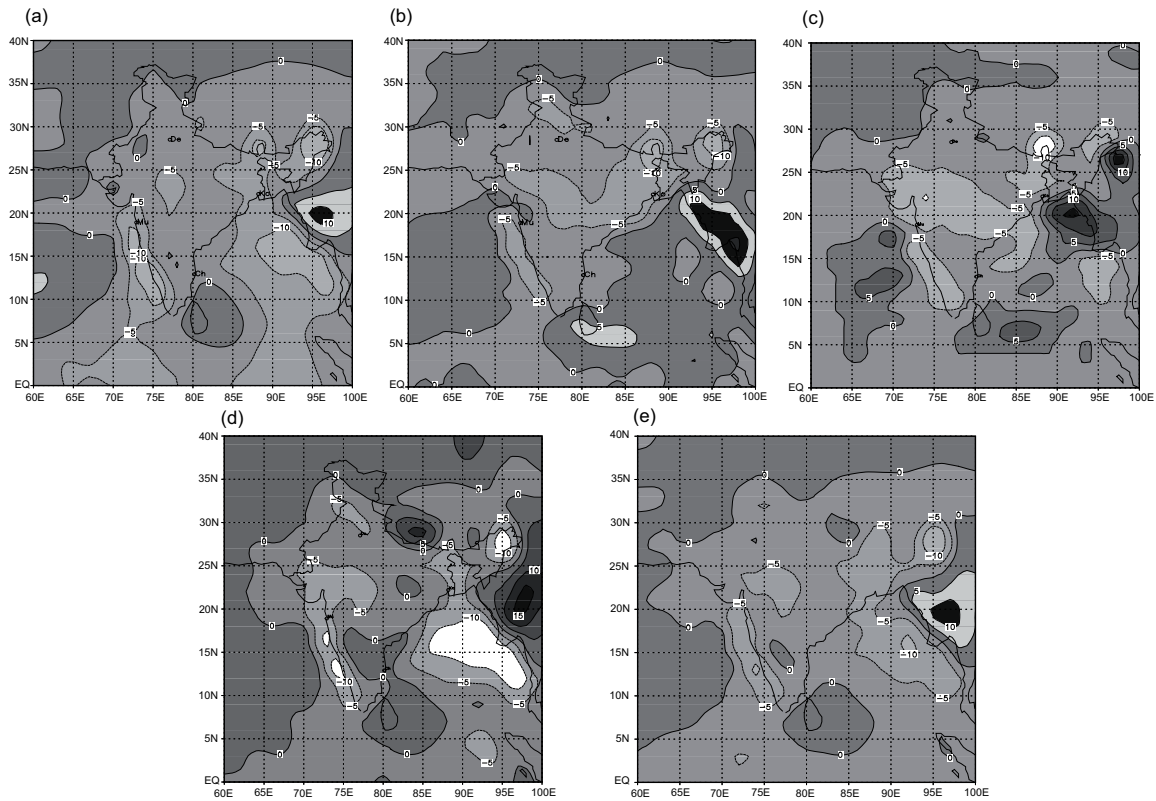
Fig. 5. Spatial distribution of season's (1 June to 30 September 2006) mean error (Forecast-analysis) in mm day-1 based on daily day-1 forecasts of (a) LAM, (b) MM5 (IMD), (c) MM5 (NCMRWF), (d) T-80 and (e) ensemble.
