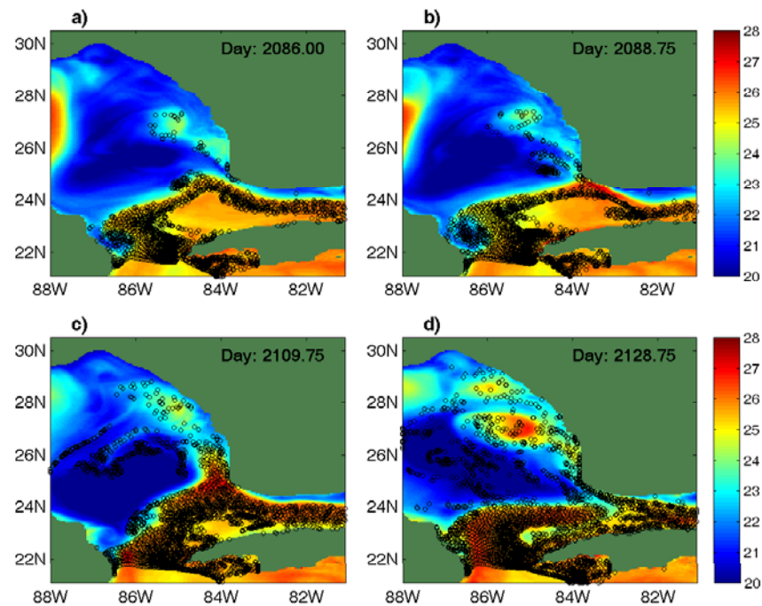
Fig. 4. Synoptic maps of 95-1000 m layer-averaged temperature and particle locations from a Gulf of México numerical simulation using the Navy Coastal Ocean Model. Colors represent temperature in Celsius and black dots represent particles seeded in the Yucatán Channel with a uniform particle density.
