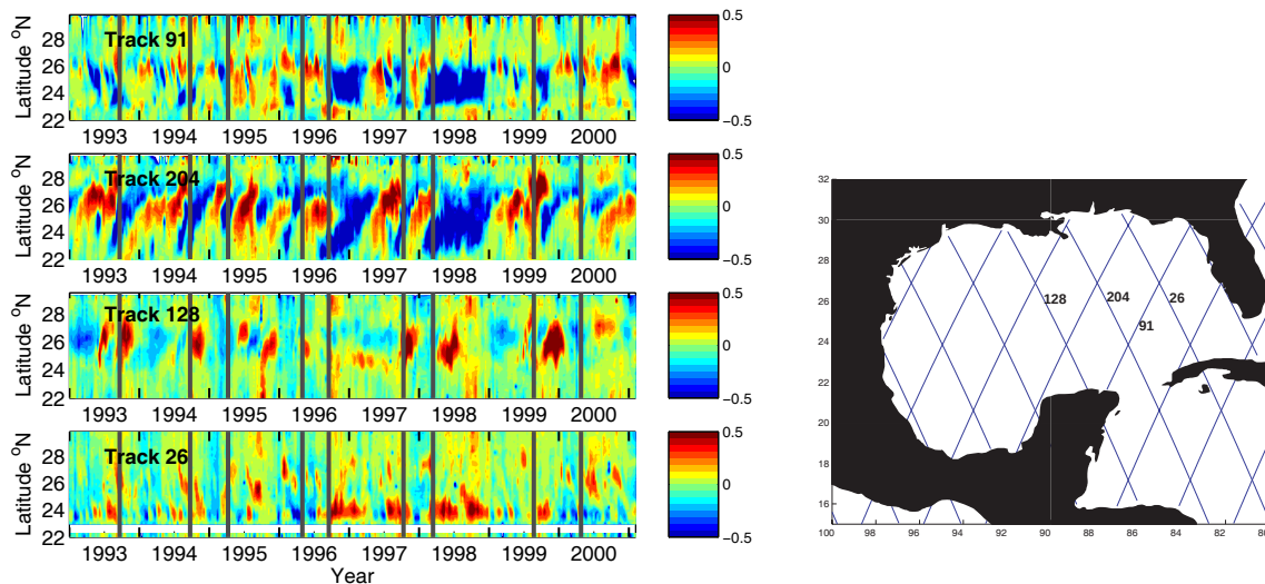
Fig. 3. Sea surface height anomaly along Topex/Poseidon tracks. Thick lines indicate the moment of separation of Loop Current eddies following Sturges and Leben (2000) and Sturges (personal communication). The track locations are indicated in the map.
